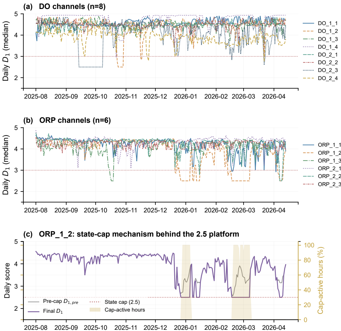
Figure 7. Daily sensor-health trajectories and state-cap interpretation
